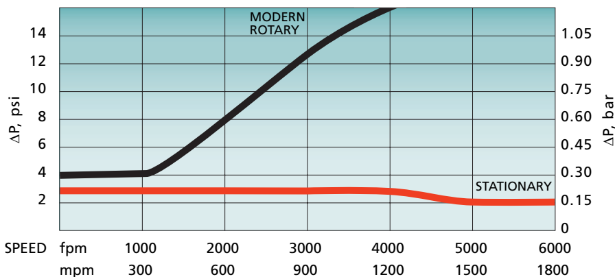
OPERATING DIFFERENTIAL PRESSURE
