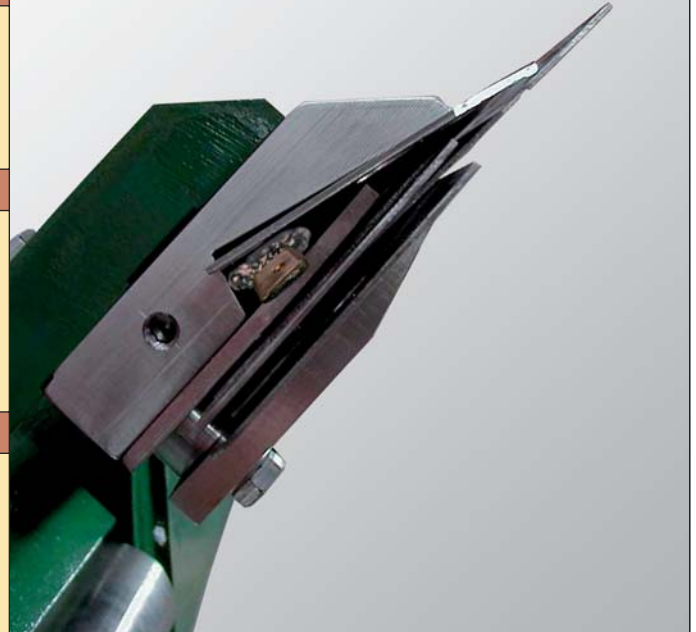
Conformatic L blade holder mounted to doctor.
